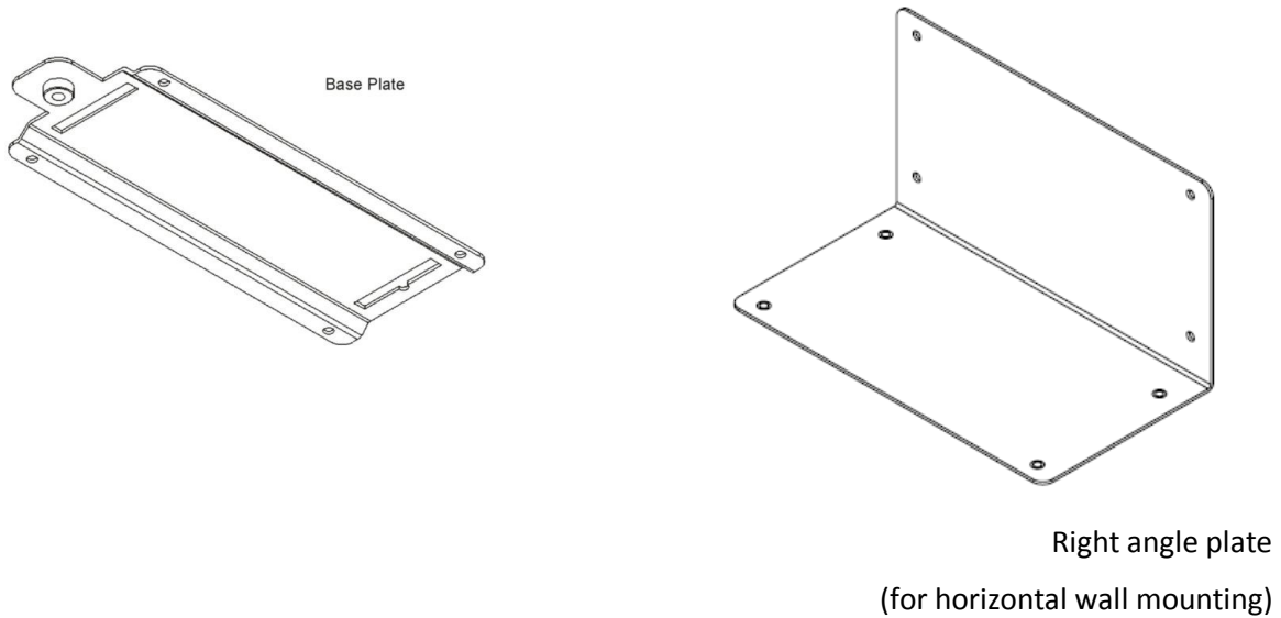
Figure 14 Mounting Plates
