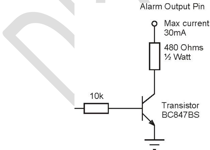
Figure 15 - Alarm Input/Output Wiring
