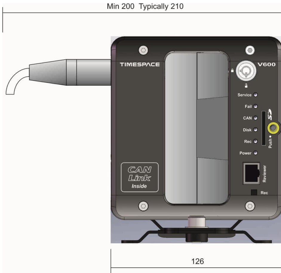
Figure 13 - V600 Front Panel Measurement Data
