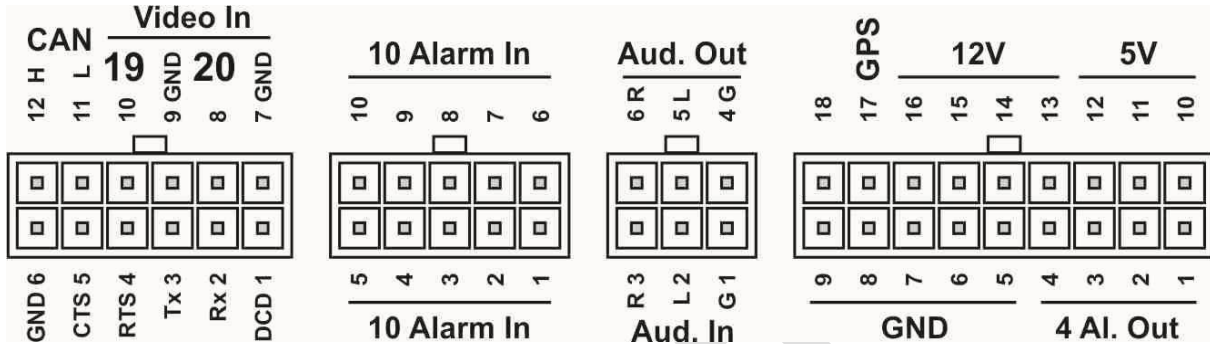
Figure 10 V600 Molex Side Panel Connectors
