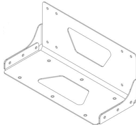
Right angle plate for horizontal wall mounting
