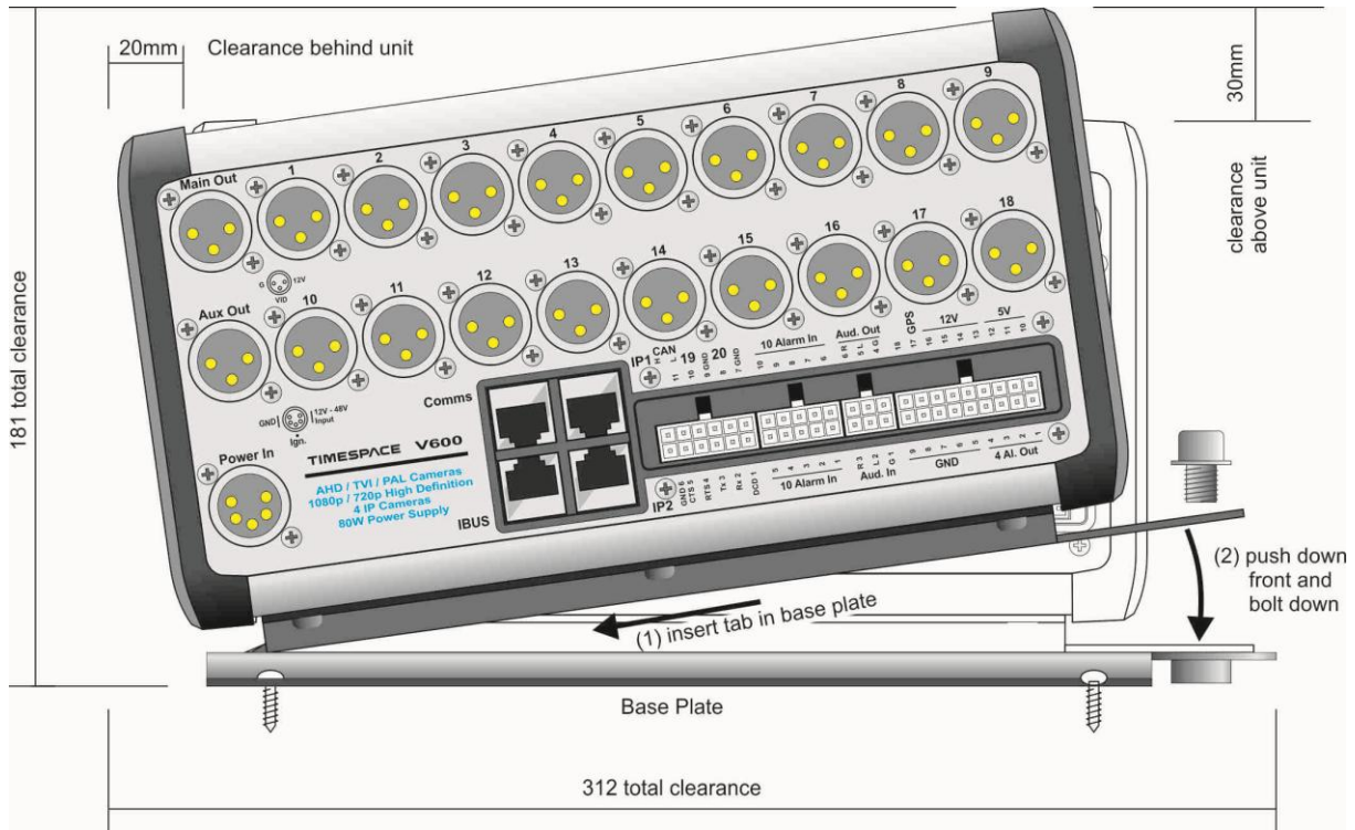
Figure 14 Mounting Plates
